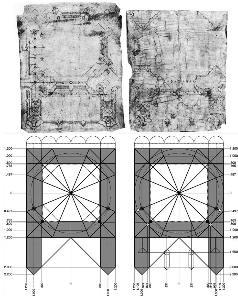
Fig. 2a (upper left). Plan drawing of Ulm Minster's west tower, from Ulm, Archiv des Münsterbauamtes. Photograph: Friedrich, "Die Risse zum Hauptturm."
