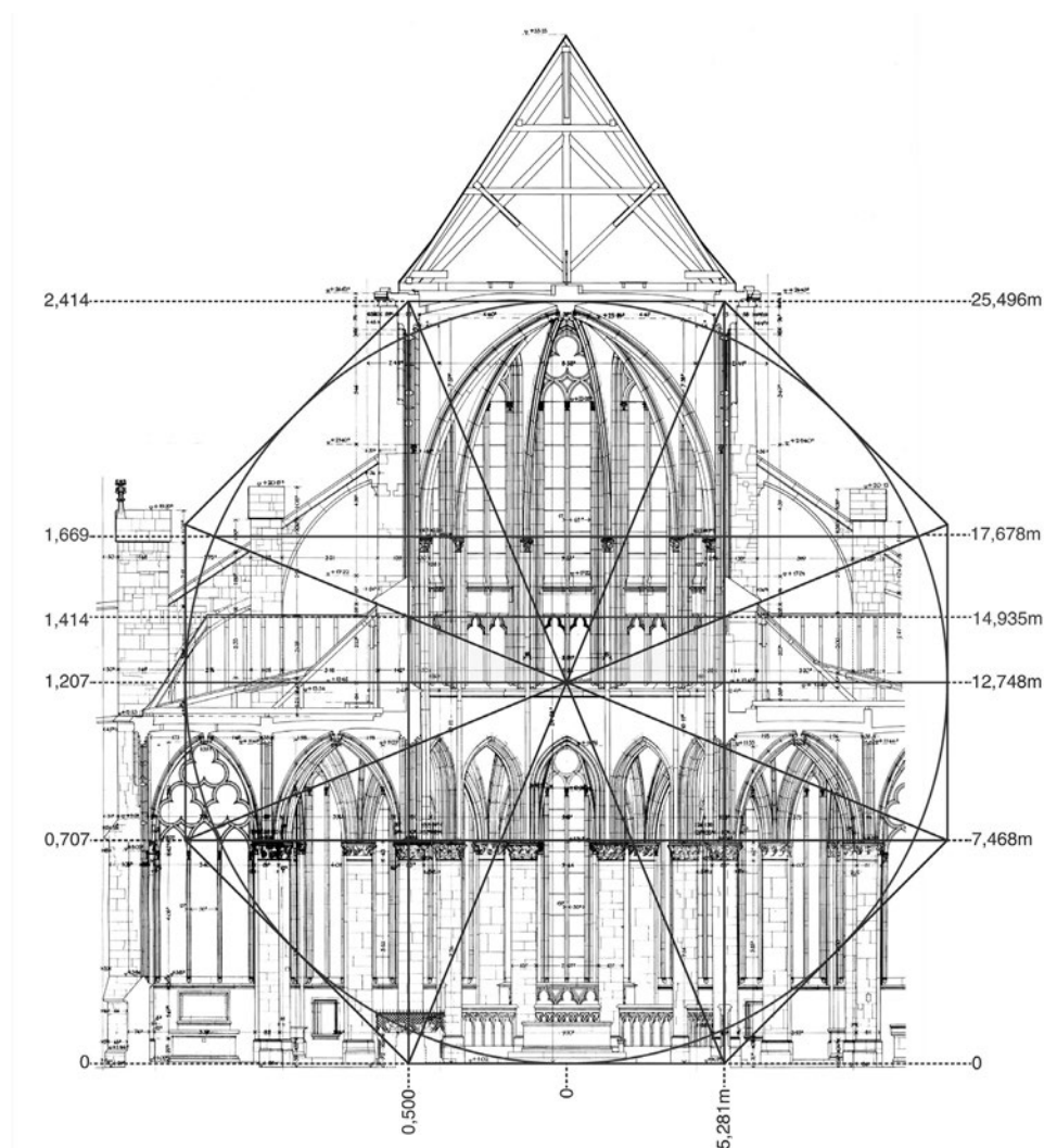
Fig. 10. Altenberg, choir section of Cistercian church, after Albert Steinmetz (1911), as first published in Lepsky and Nussbaum, Gotische Konstruktion , vol. 1, with geometrical overlay by the author.
