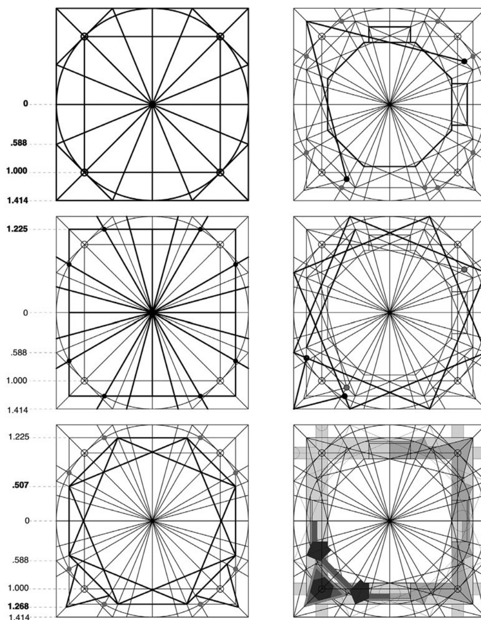
Figs. 6a-f. Successive stages in geometrical development of Freiburg upper tower cross-section. Original graphics by the author.
