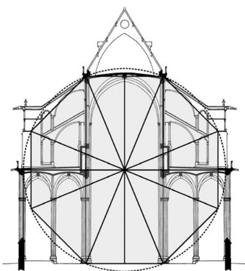
Fig. 9a. Clermont-Ferrand Cathedral, choir section, drawn by D. Fiegenschue after Henri du Ranquet (source: Davis, "The Choir of the Cathedral of Clermont-Ferrand," Fig. 6 therein), with geometrical overlay by the author.
