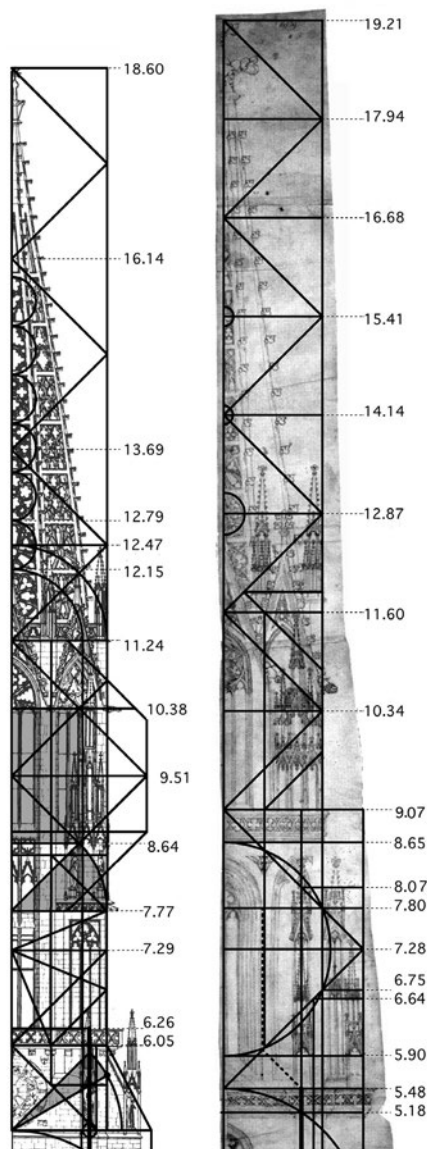
Fig. 5a. Elevation of Freiburg tower superstructure, with geometrical overlay by the author. Photograph: Freiburger Münsterbauverein e.V.
