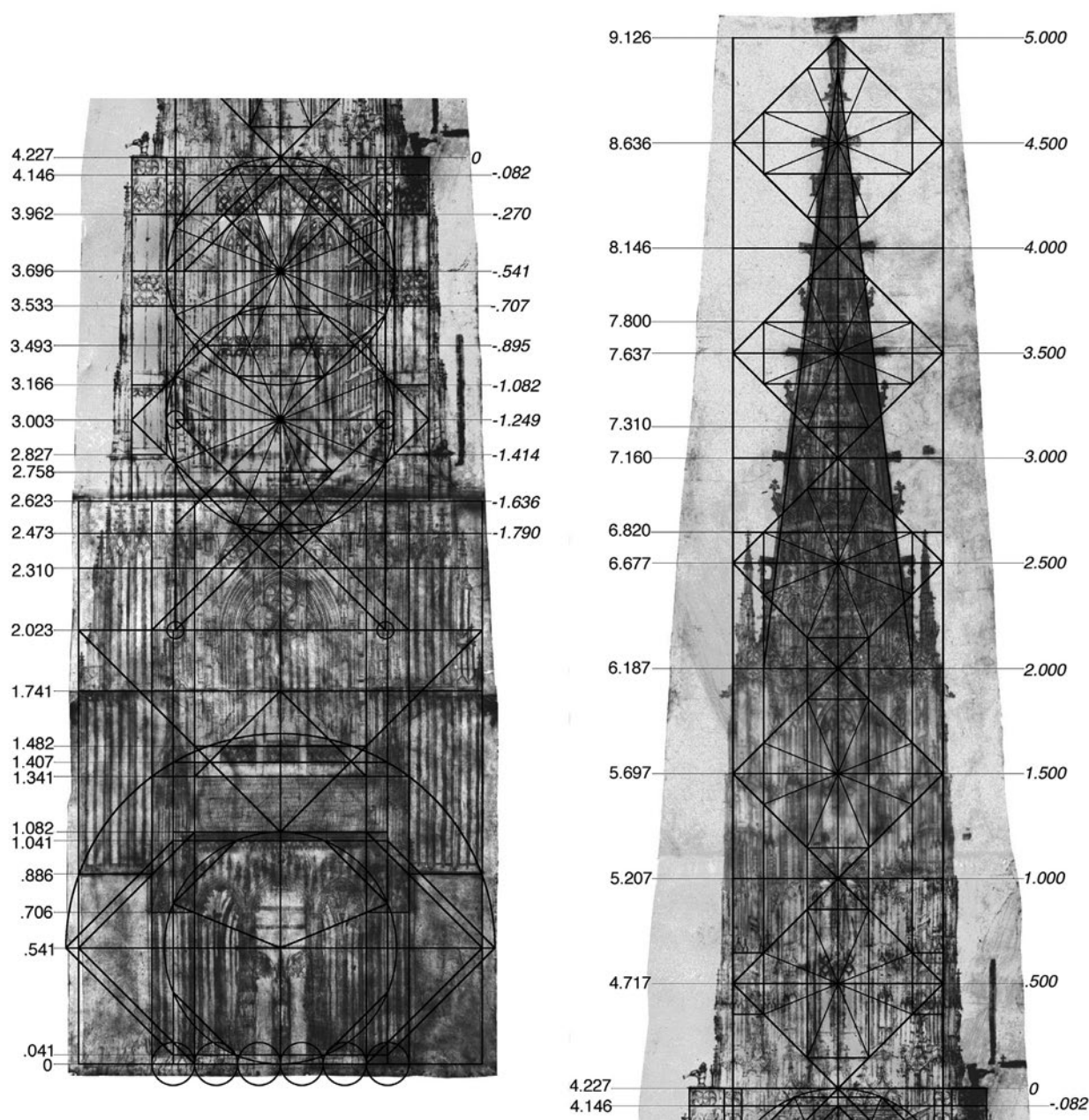
Fig. 3. Elevation drawing of Ulm Minster's west tower (Ulm Riss C), by Matthäus Böblinger, c. 1477, with geometrical overlay by the author. Photograph: Stefan Roller and Ulm, Stadtmuseum.
