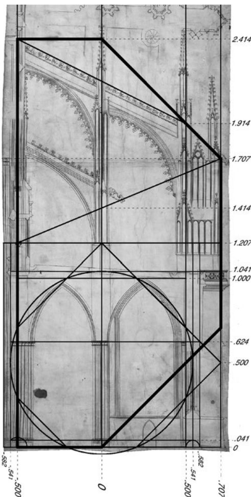
Fig. 7. Drawing 16.821 showing section of Prague Cathedral, with geometrical overlay by the author. Photograph: Vienna, Kupferstichkabinett der Akademie der bildenden Künste.
